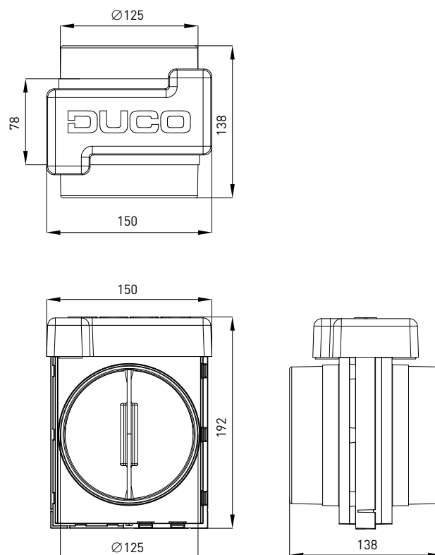
Clapet multizone DucoBox Energy Comfort (Plus) Ø125
