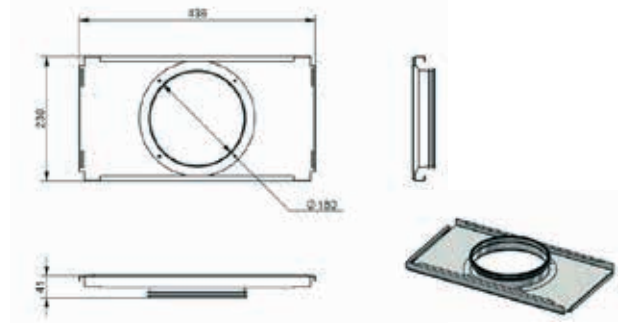
CW-K 420 Kit de montage ComfoAir Q350/450 (DN180)
