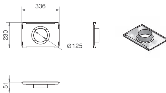
CW-K 320 Kit de montage ComfoD 250
