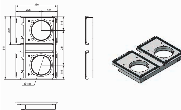
CW-K 320 Kit de montage ComfoAir Q350
