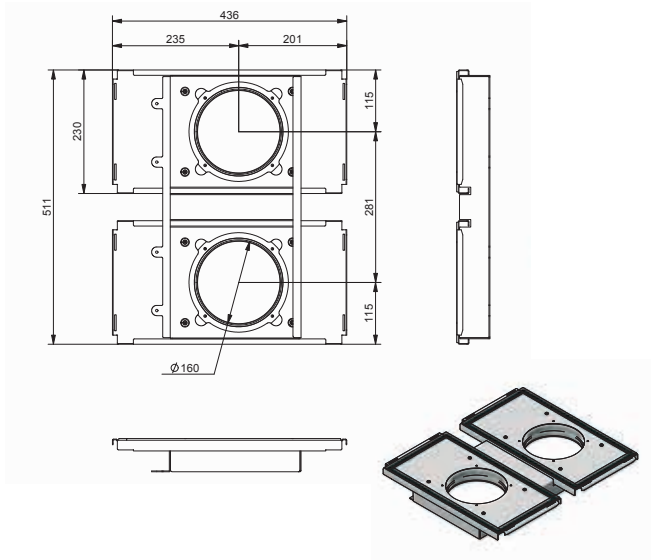
CW-K 420 Kit de montage ComfoAir Q350
