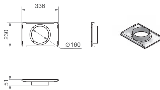
CW-K 320 Kit de montage ComfoAir Q350
