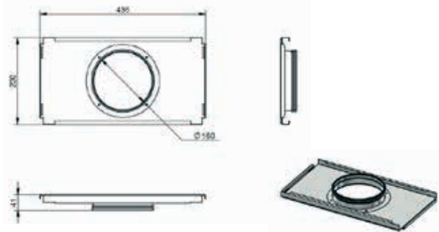
CW-K 420 Kit de montage ComfoAir Q350
