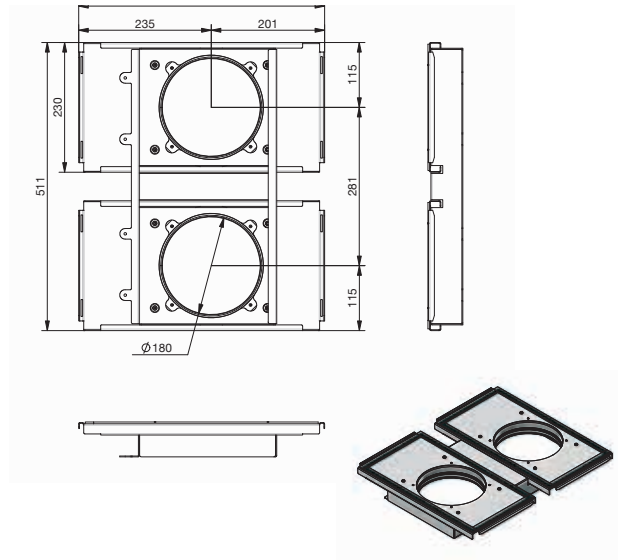
CW-K 420 Kit de montage ComfoAir Q350/450 (DN180)
