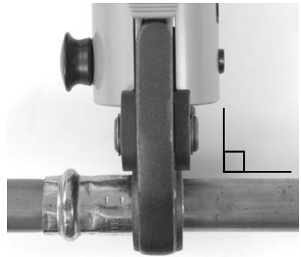
Figure 7 – Jaws Square to Fitting
